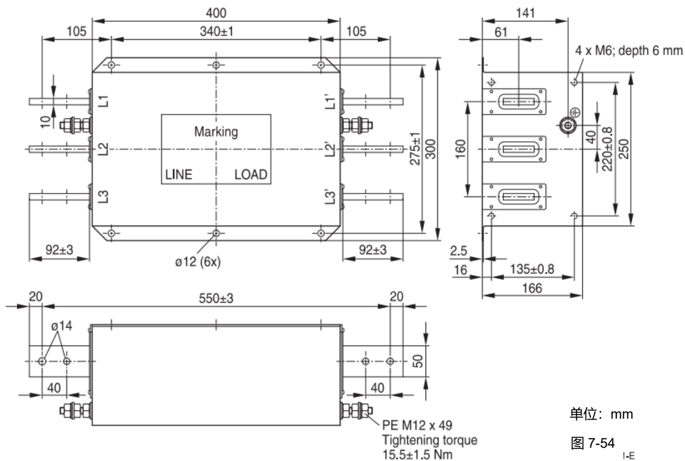
EMC 滤波器型号: B84143B1600S020
