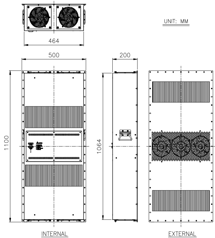
Dimension drawing
