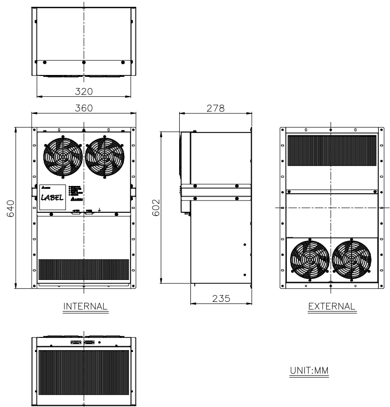
Dimension drawing
