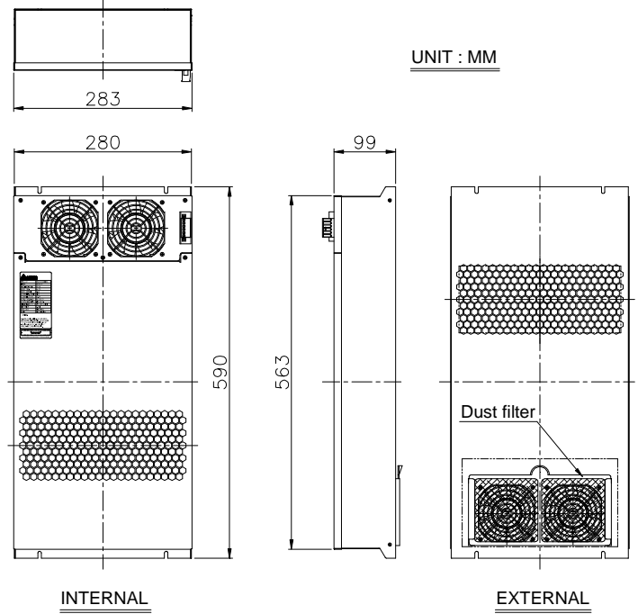
Dimension drawing
